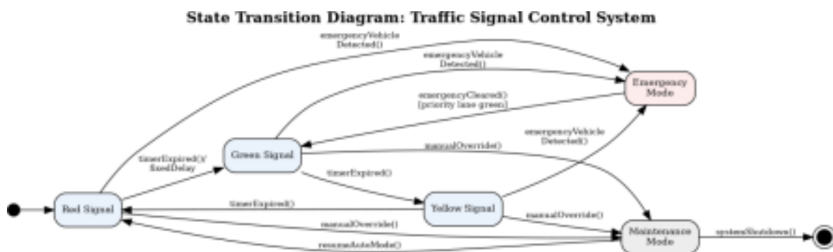
Figure 4: State Transition Diagram for the Traffic Signal Control System, showing the normal timer driven cycle plus emergency and maintenance interrupt states.
